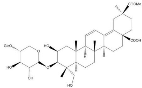
Structure:
